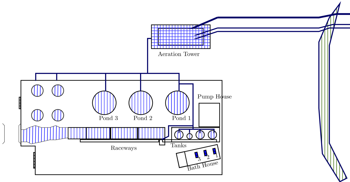
Figure 2.6: Mbona Hatcheries Water Reticulation System.
